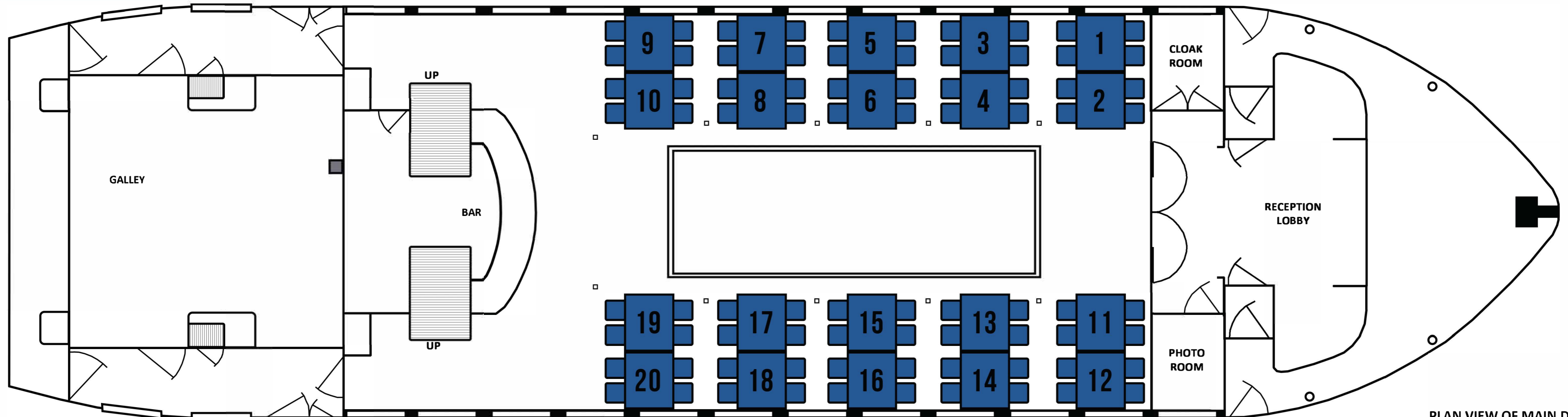
PLAN VIEW OF MAIN DECK
